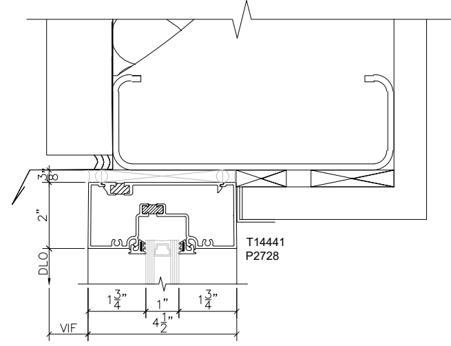
6 STOREFRONT HEAD SCALE : 3" = 1'-0" ARCH REF: 1/A3.3
