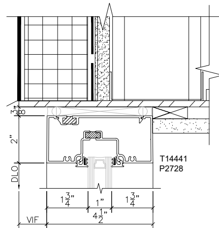
8 STOREFRONT HEAD SCALE : 3" = 1'-0" ARCH REF: 1/A3.2
