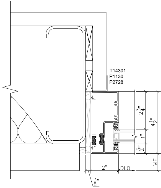
1 503 STOREFRONT JAMB SCALE : 3" = 1'-0 ARCH REF: 1/A3.3
