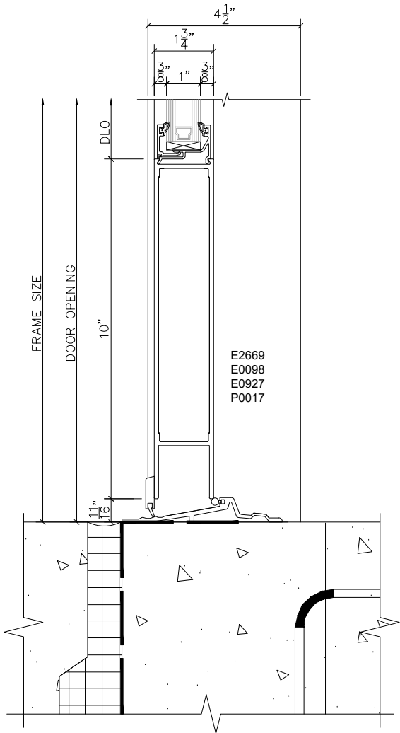
5 DOOR SILL SCALE : 3" = 1'-0" ARCH REF: 1/A3.2
