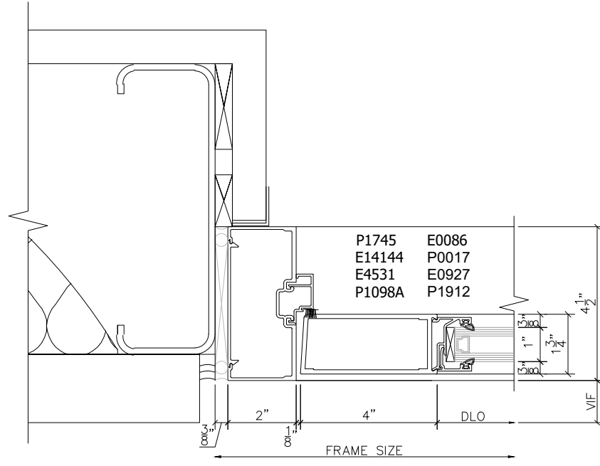
3 503 DOOR JAMB SCALE : 3" = 1'-0 ARCH REF: 1/A3.3
