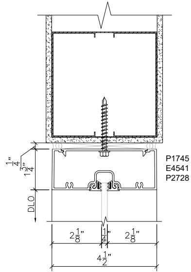
6 STOREFRONT HEAD 600 SCALE : 3" = 1'-0" ARCH REF: XXX
