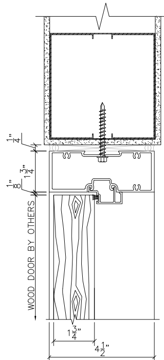
8 DOOR HEAD 600 SCALE : 3" = 1'-0" ARCH REF: XXX
