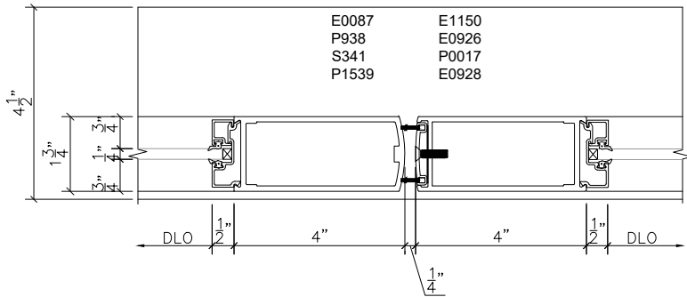
5 DOOR MEETING STILE 601 SCALE : 3" = 1'-0 ARCH REF: xxx
