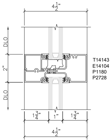
2 STOREFRONT HORIZONTAL SCALE : 3" = 1'-0" ARCH REF: XXX
