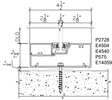
3 STOREFRONT SILL 600 SCALE : 3" = 1'-0" ARCH REF: 3/A/701
