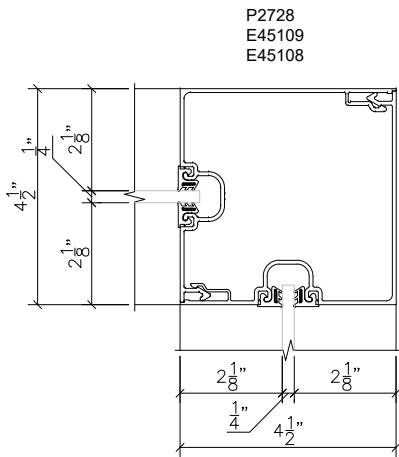
3 STOREFRONT JAMB 601 SCALE : 3" = 1'-0 ARCH REF: XXX
