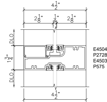
2 STOREFRONT HORIZONTAL 600 SCALE : 3" = 1'-0" ARCH REF: 3/A/701
