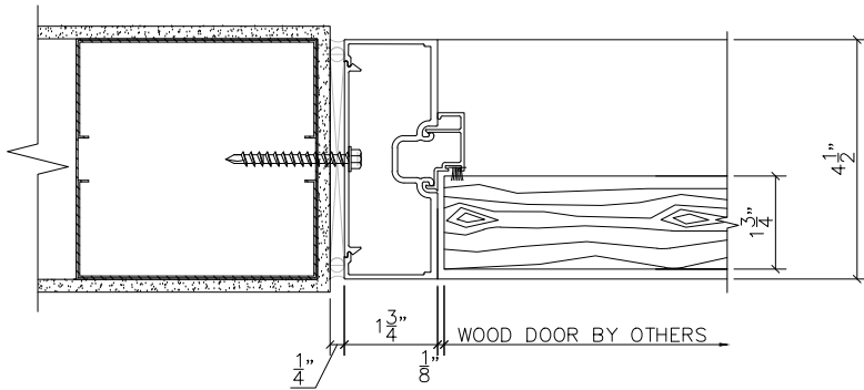
7 DOOR JAMB 601 SCALE : 3" = 1'-0 ARCH REF: xxx
