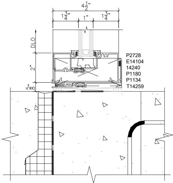
3 DOOR SILL SCALE : 3" = 1'-0" ARCH REF: 1/A3.2
