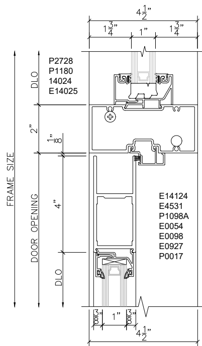
4 DOOR HEAD SCALE : 3" = 1'-0" ARCH REF: XXX
