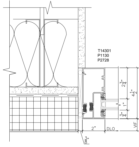
4 503 STOREFRONT JAMB SCALE : 3" = 1'-0 ARCH REF: 14/A5.4
