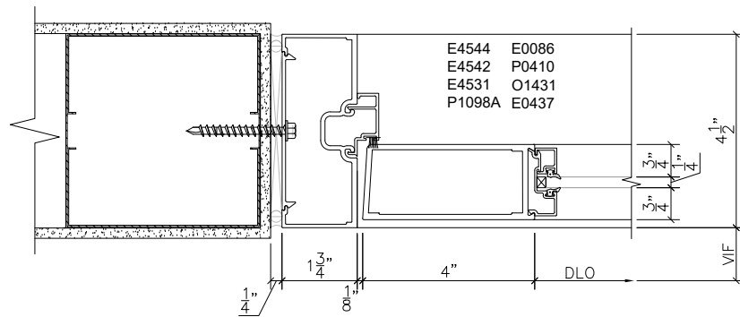
6 DOOR JAMB 601 SCALE : 3" = 1'-0 ARCH REF: xxx
