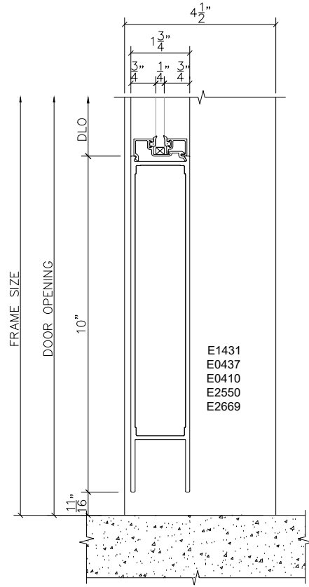
5 DOOR SILL 502 SCALE : 3" = 1'-0" ARCH REF: XXX
