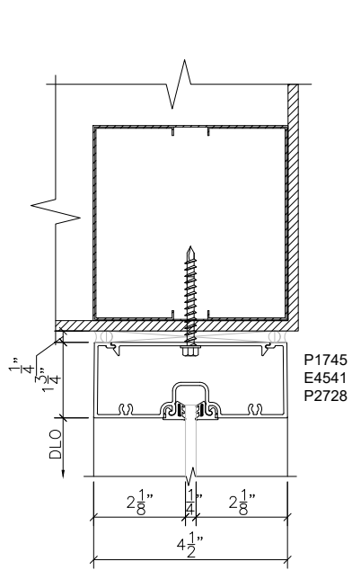
1 STOREFRONT HEAD 600 SCALE : 3" = 1'-0" ARCH REF: XXX
