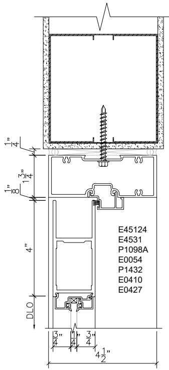
7 DOOR HEAD 600 SCALE : 3" = 1'-0" ARCH REF: XXX
