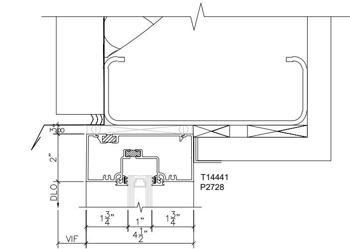
1 STOREFRONT HEAD SCALE : 3" = 1'-0" ARCH REF: 1/A3.3
