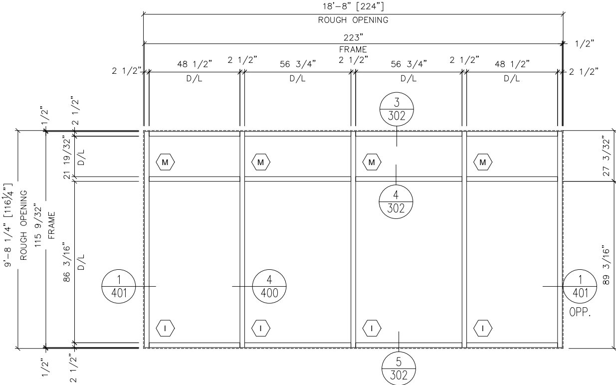
W14 22-THUS FRAMING: KAWNEER 1600SS (2 1/2" X 6") ARCH REF: W14A-603
