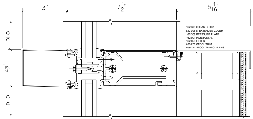
2 301 CURTAIN WALL HORIZONTAL SCALE : 3" = 1'-0 ARCH REF: 4/A303
