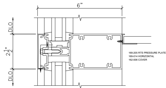
4 302 CURTAIN WALL HORIZONTAL SCALE : 3" = 1'-0 ARCH REF: XXX
