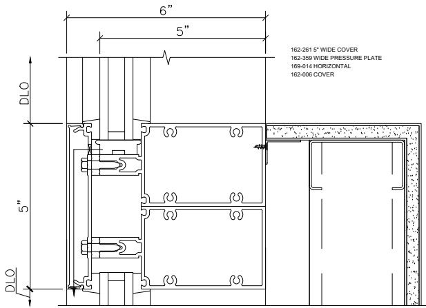
2 CURTAIN WALL HORIZONTAL 303 SCALE : 3" = 1'-0 ARCH REF: XXX
