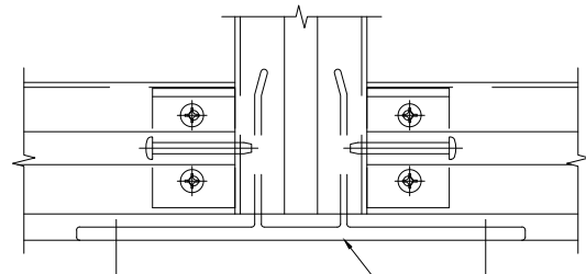
5 FRONT VIEW OF MULLION DETAIL ARCH. REF: Scale: 6"=1'
