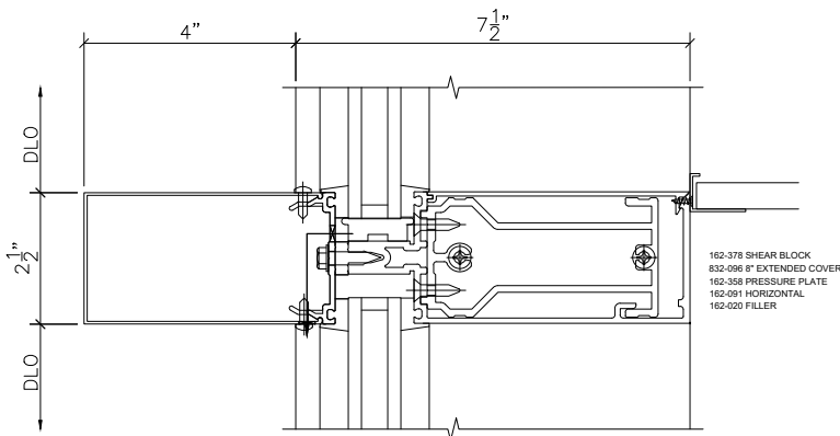
4 301 CURTAIN WALL HORIZONTAL SCALE : 3" = 1'-0 ARCH REF: XXX
