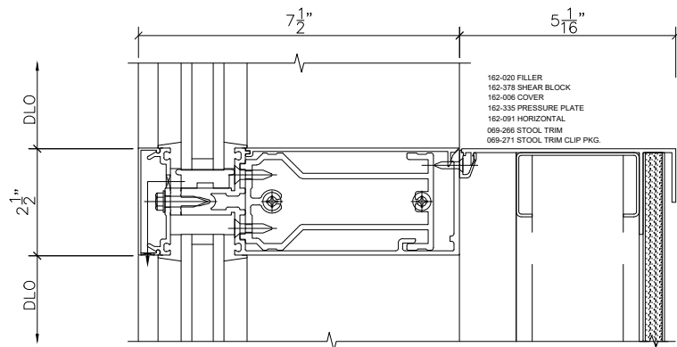
1 301 CURTAIN WALL HORIZONTAL SCALE : 3" = 1'-0 ARCH REF: 4/A303
