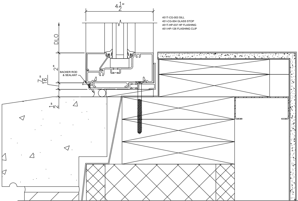
2 304 STOREFRONT HORIZONTAL SCALE : 3" = 1'-0" ARCH REF: XXX
