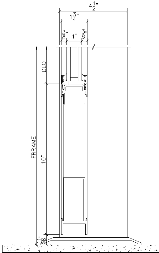
5 304 DOOR SILL SCALE : 3" = 1'-0" ARCH REF: XXX
