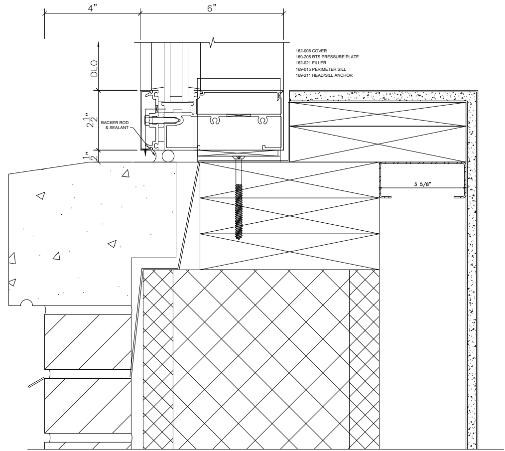
7 CURTAIN WALL SILL 303 SCALE : 3" = 1'-0 ARCH REF: 3/A3.02
