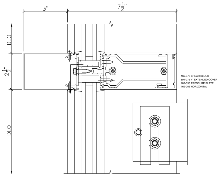
5&7 301 CURTAIN WALL HORIZONTAL SCALE : 3" = 1'-0 ARCH REF: XXX
