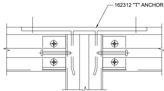
4 FRONT VIEW OF MULLION DETAIL ARCH. REF: Scale: 6"=1'
