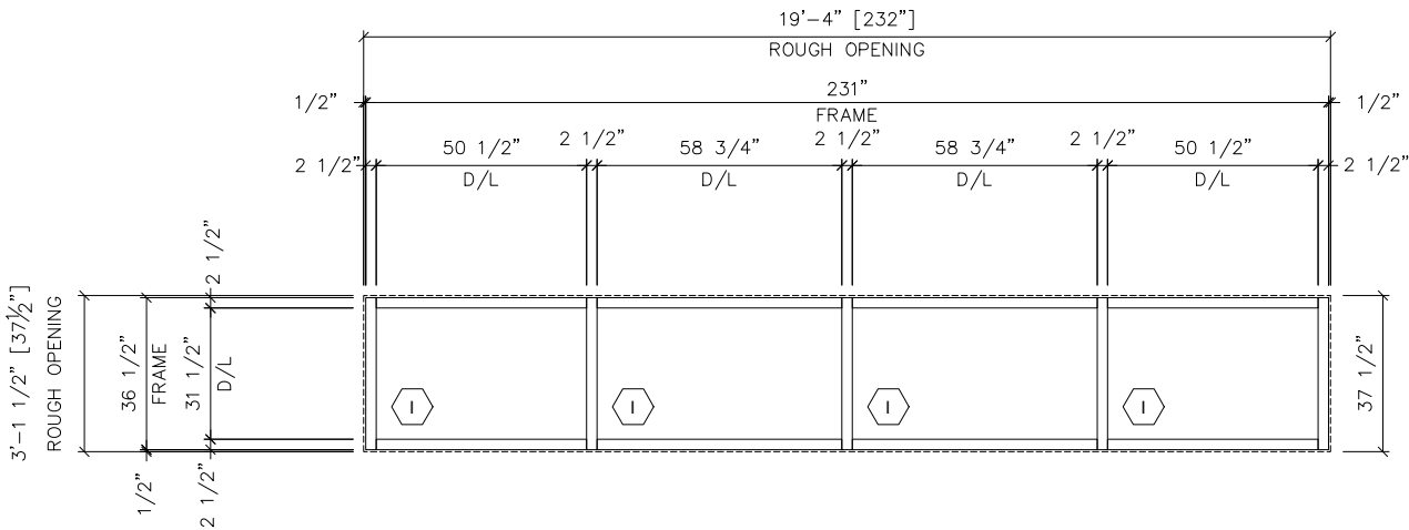
W13 4-THUS FRAMING: KAWNEER 1600SS (2 1/2" X 6") ARCH REF: W13A/A-603 @ OPPOSITE HAND
