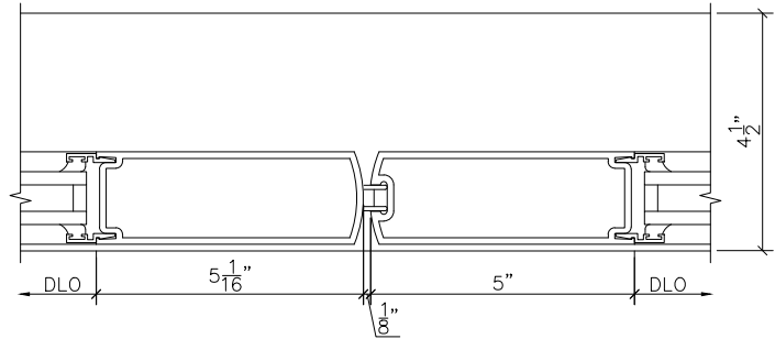
1 DOOR MEETING STILE 403 SCALE : 3" = 1'-0 ARCH REF: XXX
