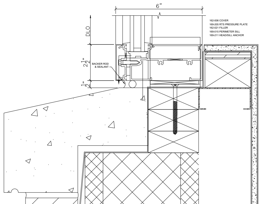
5 302 CURTAIN WALL SILL SCALE : 3" = 1'-0 ARCH REF: 3/A3.02
