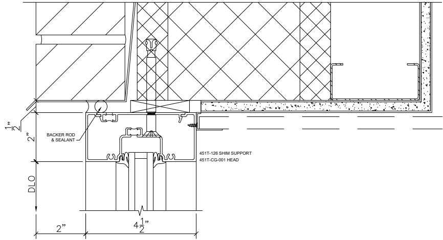
1 304 STOREFRONT HEAD SCALE : 3" = 1'-0" ARCH REF: 3/A3.02
