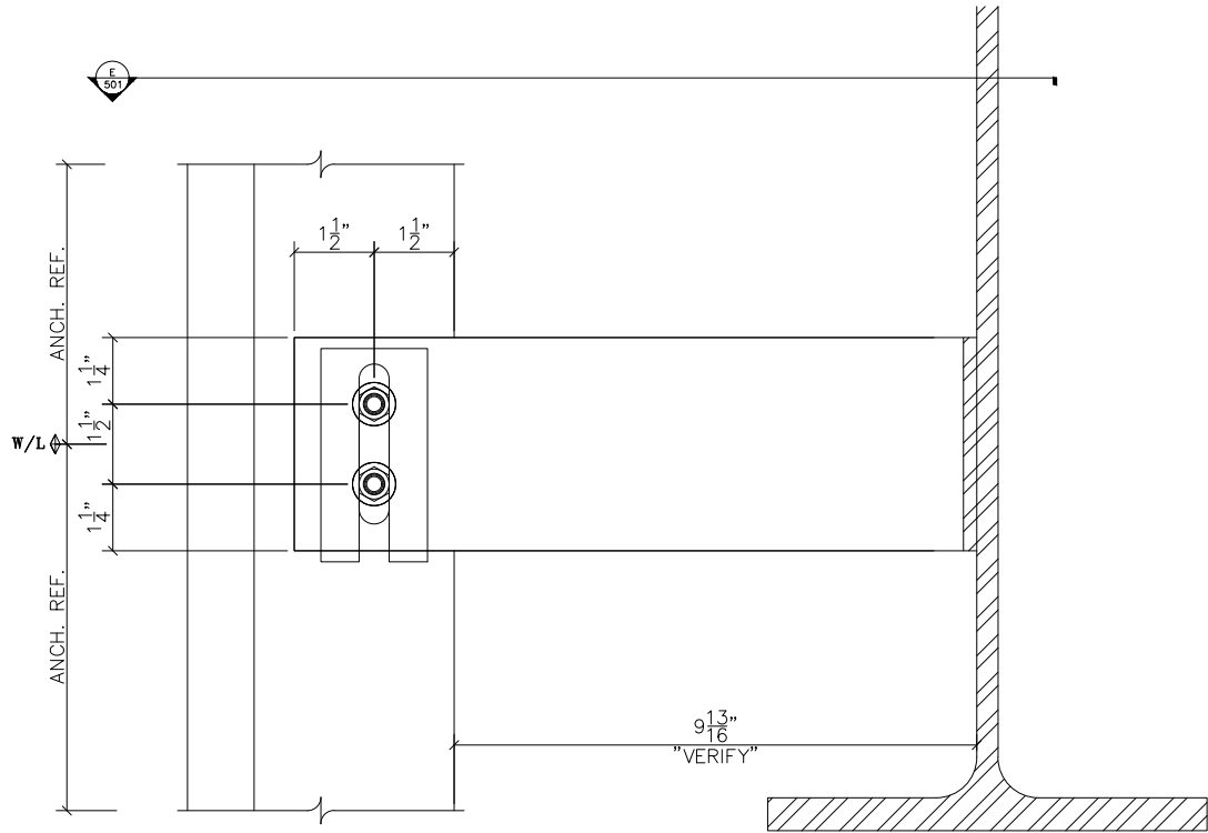
1 ANCHOR DETAIL 502 SCALE : 3" = 1'-0 ARCH REF: XXX
