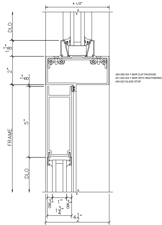
4 304 DOOR HEAD SCALE : 3" = 1'-0" ARCH REF: XXX
