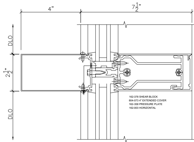
6 301 CURTAIN WALL HORIZONTAL SCALE : 3" = 1'-0 ARCH REF: XXX
