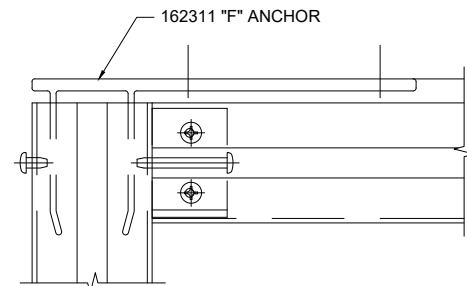
6 FRONT VIEW OF MULLION DETAIL ARCH. REF: Scale: 6"=1'
