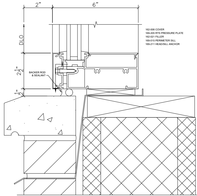
5 CURTAIN WALL SILL 303 SCALE : 3" = 1'-0 ARCH REF: 3/A3.02
