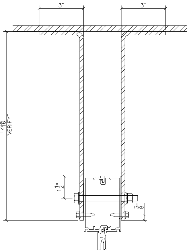
D SECTION-DEAD LOAD ANCHOR LAYOUT SCALE : 3" = 1'-0" ARCH REF: XXX
