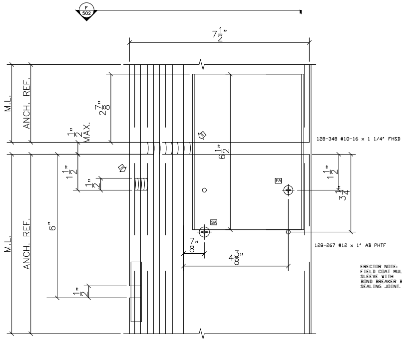
2 SPLICE DETAIL 502 SCALE : 3" = 1'-0 ARCH REF: XXX
