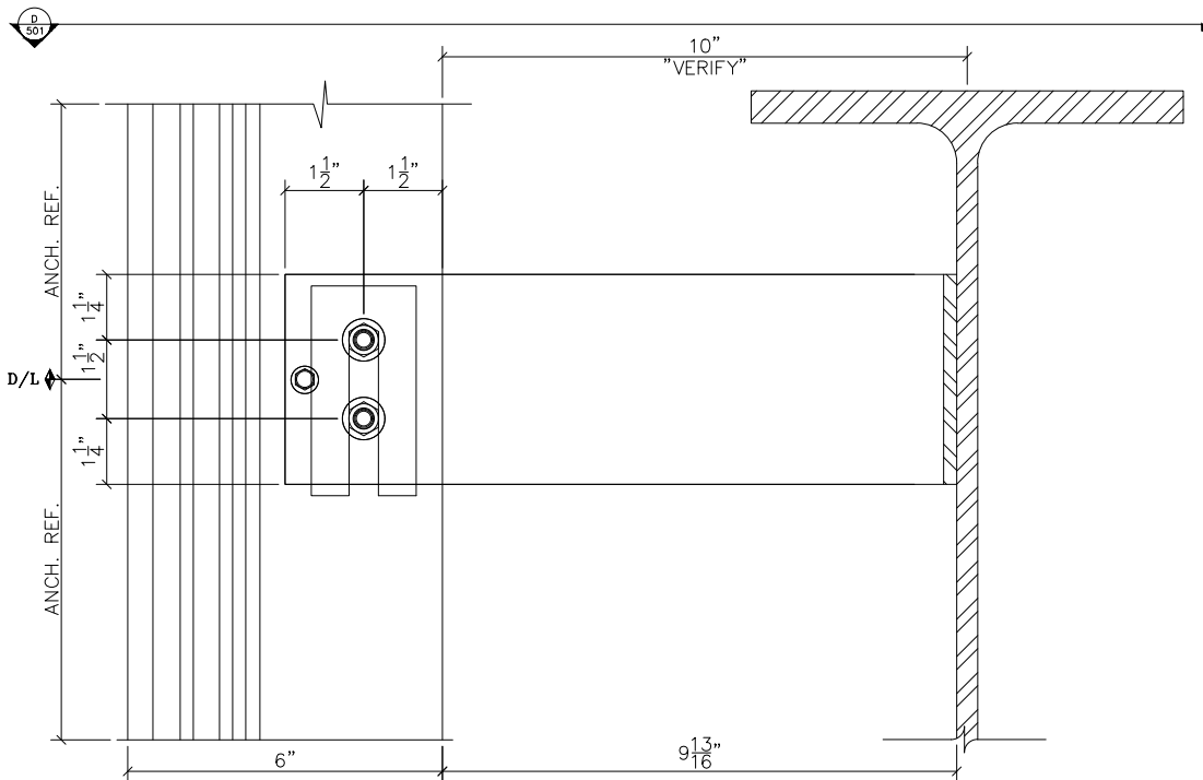
1 ANCHOR DETAIL SCALE : 3" = 1'-0" ARCH REF: XXX
