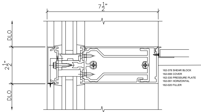
3 301 CURTAIN WALL HORIZONTAL SCALE : 3" = 1'-0 ARCH REF: 4/A303
