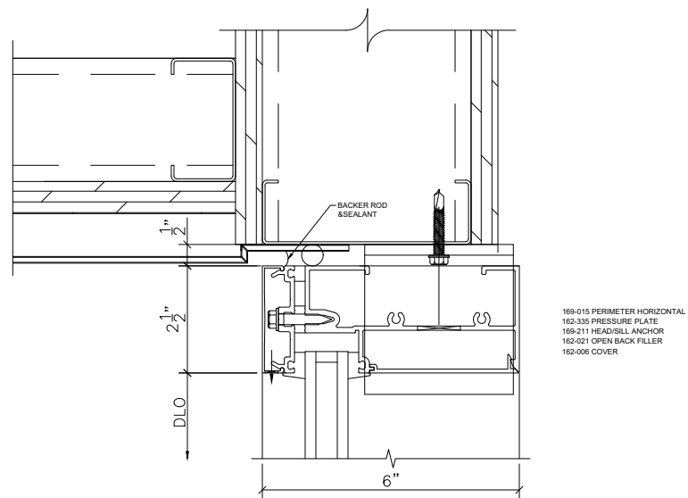
3 302 CURTAIN WALL HEAD SCALE : 3" = 1'-0 ARCH REF: 3/A3.02
