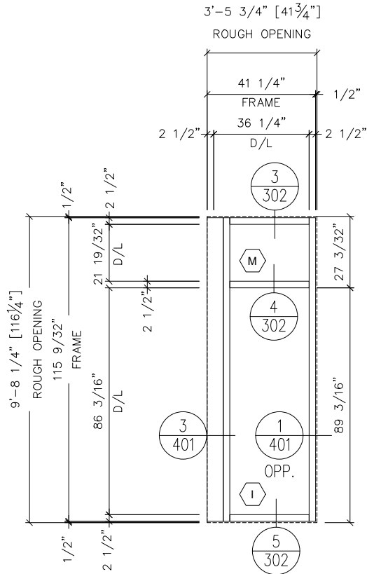
W13 4-THUS FRAMING: KAWNEER 1600SS (2 1/2" X 6") ARCH REF: W13A/A-603
