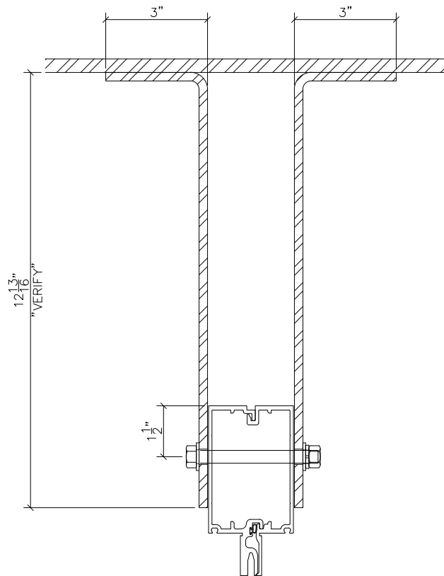
E SECTION-WIND LOAD ANCHOR LAYOUT SCALE : 3" = 1'-0" ARCH REF: XXX
