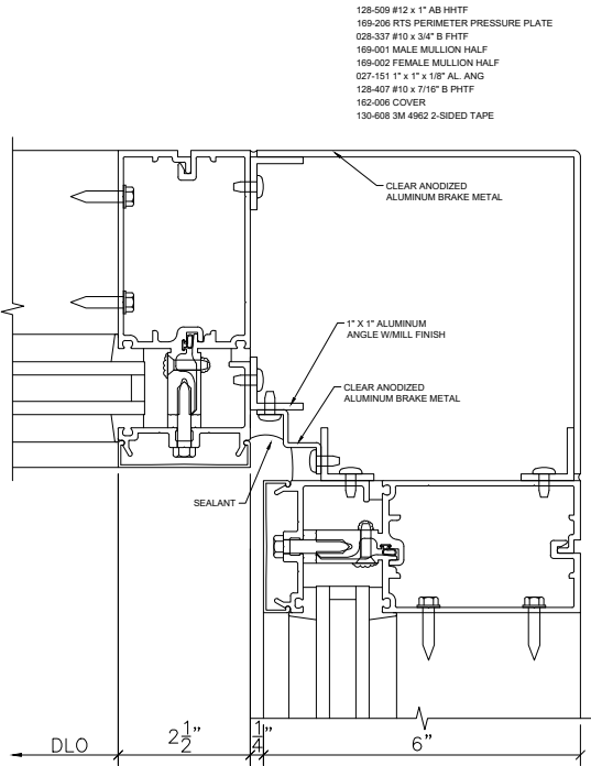
2 CURTAIN WALL INSIDE-CORNER 401 SCALE : 3" = 1'-0 ARCH REF: XXX
