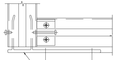
7 FRONT VIEW OF MULLION DETAIL ARCH. REF: Scale: 6"=1'
